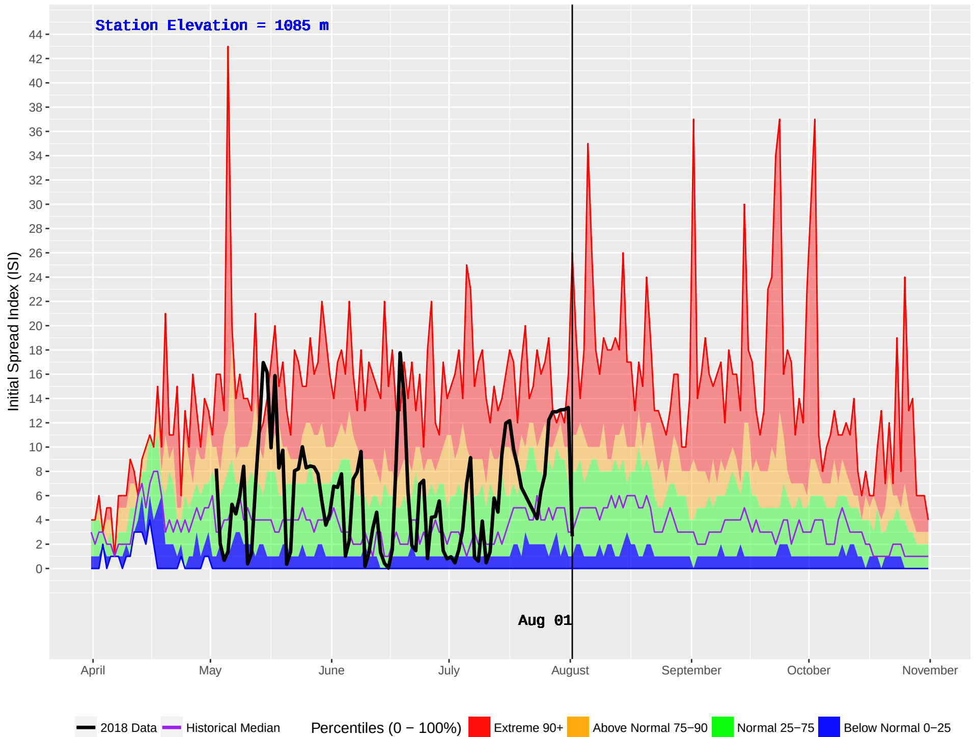
TAUTRI (206) : Historical (1970–2016) and Current (2018) Daily Initial Spread Index (ISI)
